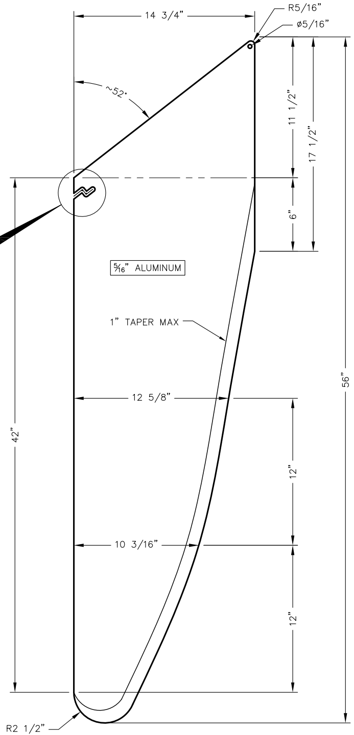
PLAN CENTERBOARD 1-1/2"=1'-0"
