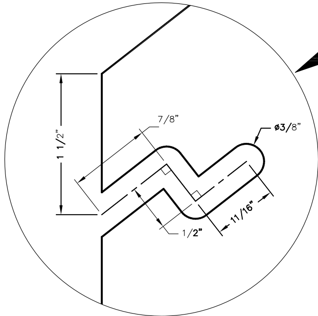
DETAIL CUTOUT 1'-0"=1'-0"
